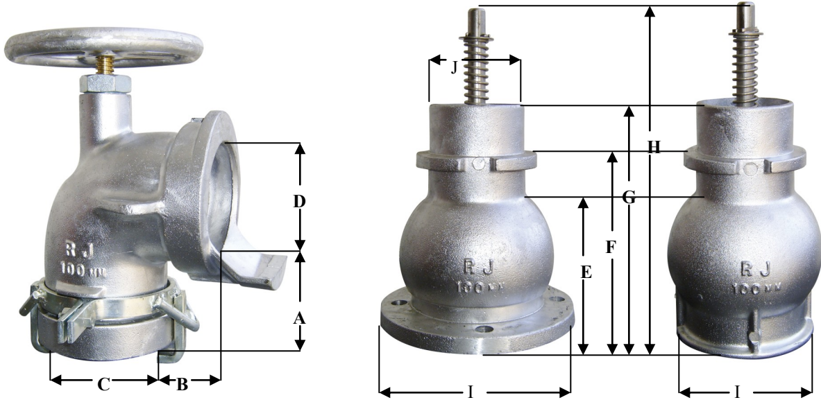
DIMENSIONS IN mm (Approx)
