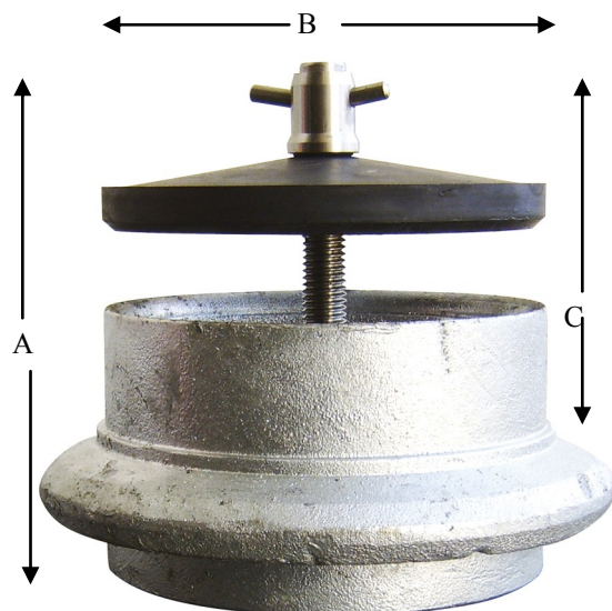
HYDRANT
